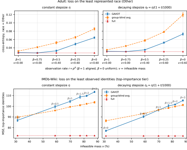
Figure 2: Loss on the least represented group, the metric the fairness target is about. Top, Adult: cross-entropy on race Other, one group of 30 out of 100, to which the category-uniform target assigns p_i = 0.2 ; the axis is the observation-rate exponent, \beta=1 aligned, \beta=0 uniform (prevalence). Bottom, IMDb-Wiki: MSE on the 20 highest-importance identities, the least observed ones once \beta > 0 , against \nu . Left panels constant stepsize, right panels decaying. Same protocol as the tables ( K=3 , H=5 , 4000 steps, tail-500 mean \pm std over 5 seeds); lower is better. Curves are the group-wise entries of the same runs as Table 1 and Fig. 1.
