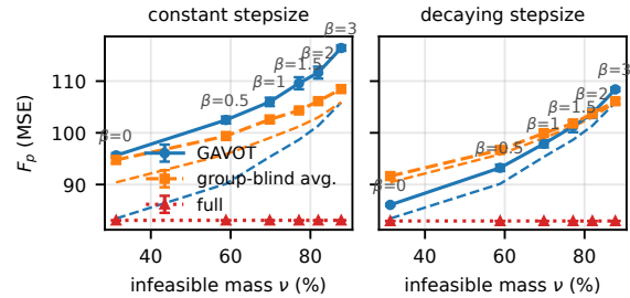
Figure 1: IMDb-Wiki severity sweep. Solid, measured tail-500 ( \pm 1 std); dashed, the exact floor \Phi(\cdot) each rule converges to. Left, constant stepsize: the optimization residual swamps the alignment gain and transport loses everywhere, even where the floors are seven units apart. Right, decaying stepsize: the residual collapses and the measured curves track their floors, so transport wins until the floors close at high \nu . The sign is set by which of the two terms of (9) dominates, not by the regime label.
