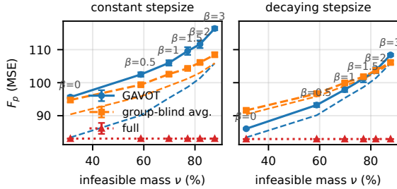
Figure 2: IMDb-Wiki severity sweep. Solid, measured tail-500 ( \pm 1 std); dashed, the exact floor \Phi(\cdot) each rule converges to. Left, constant stepsize: the optimization residual swamps the alignment gain and transport losses everywhere, even where the floors are seven units apart. Right, decaying stepsize: the residual collapses and the measured curves track their floors, so transport wins until the floors close at high \nu . The sign is set by which of the two terms of (9) dominates, not by the regime label.
