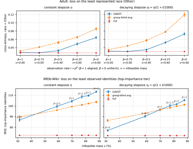
Figure 3: Loss on the least represented group, the metric the fairness target is about. Top, Adult: cross-entropy on race Other, one group of 30 out of 100, to which the category-uniform target assigns p_i = 0.2 ; the axis is the observation-rate exponent, \beta=1 aligned, \beta=0 uniform (prevalence). Bottom, IMDb-Wiki: MSE on the 20 highest-importance identities, the least observed ones once \beta > 0 , against \nu . Left panels constant stepsize, right panels decaying. Same protocol as the tables ( K=3 , H=5 , 4000 steps, tail-500 mean \pm std over 5 seeds); lower is better. Curves are the group-wise entries of the same runs as Table 1 and Fig. 2.
