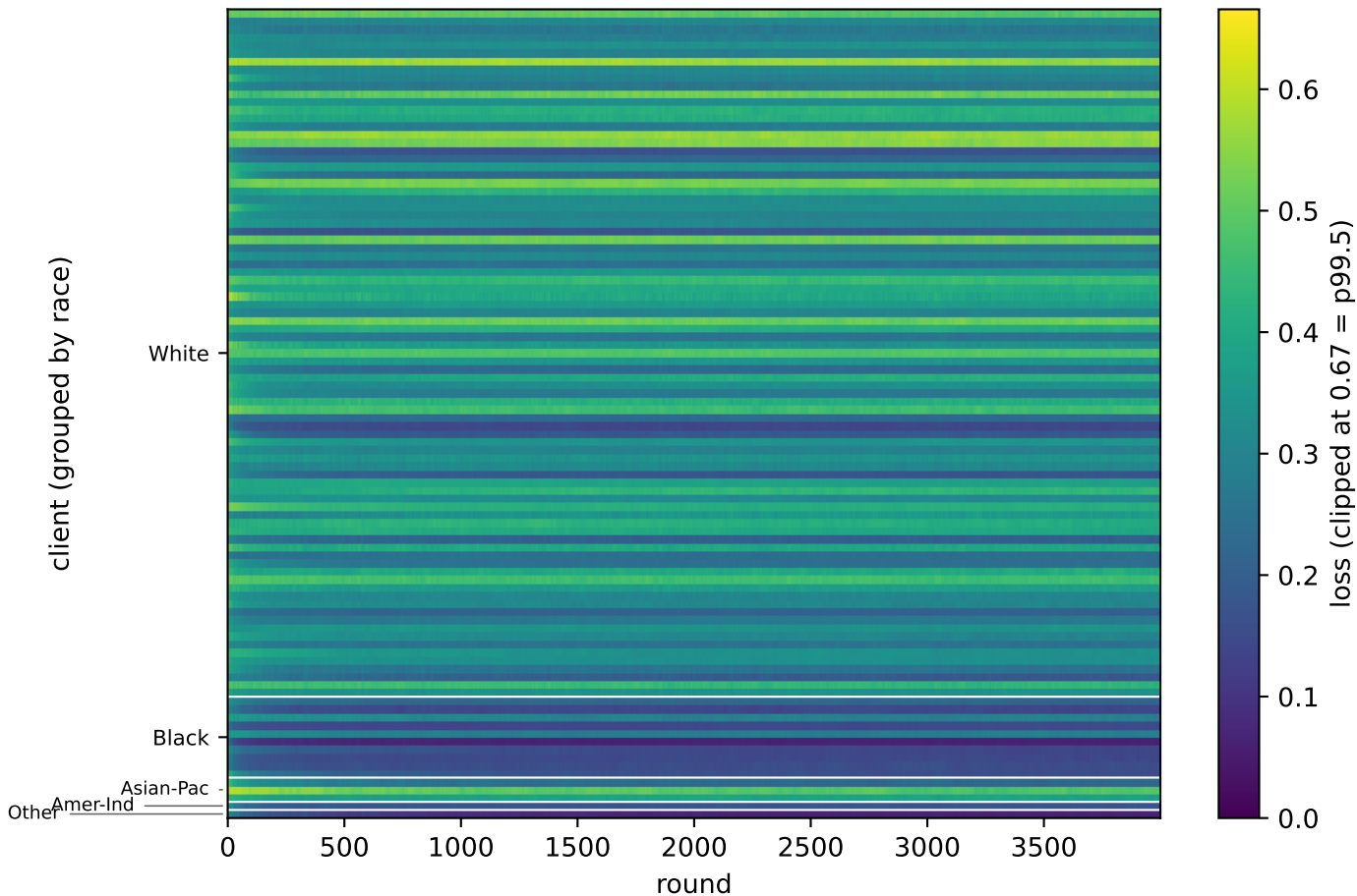
adult / infeasible — FedAVOT per-client loss (5-seed mean)
