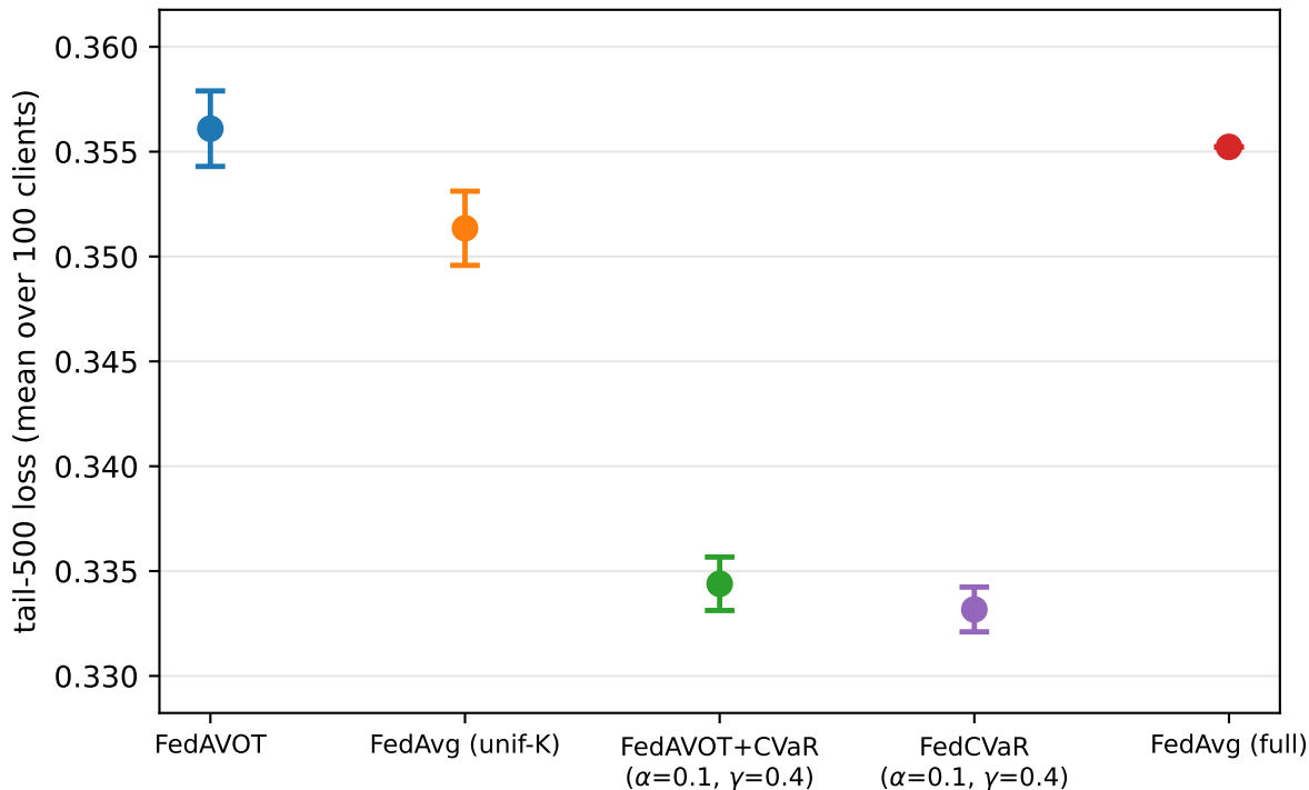
adult / feasible — overall tail-500 loss (mean \pm std, 5 seeds)
