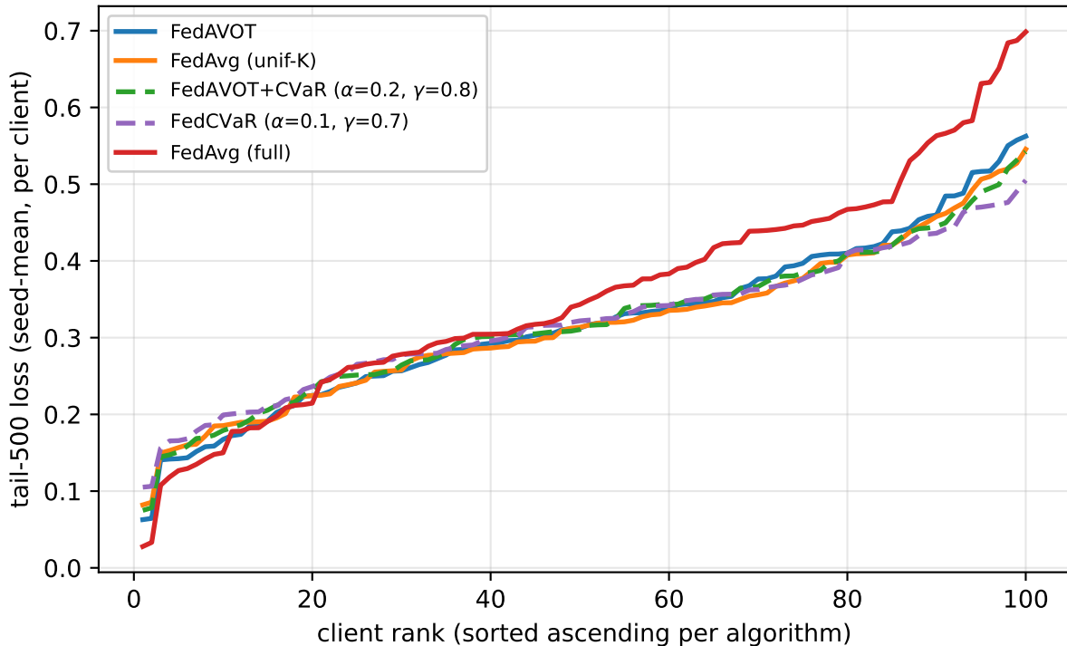
adult / infeasible — sorted per-client tail-500 loss
