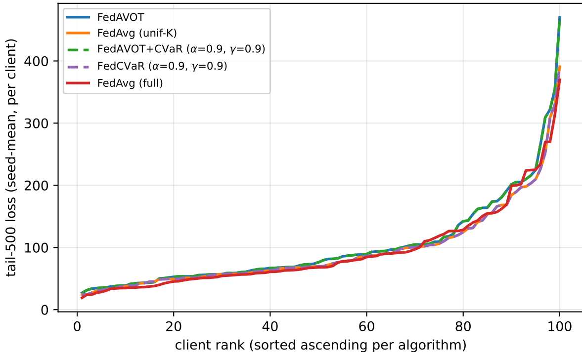
imdbwiki / infeasible — sorted per-client tail-500 loss
