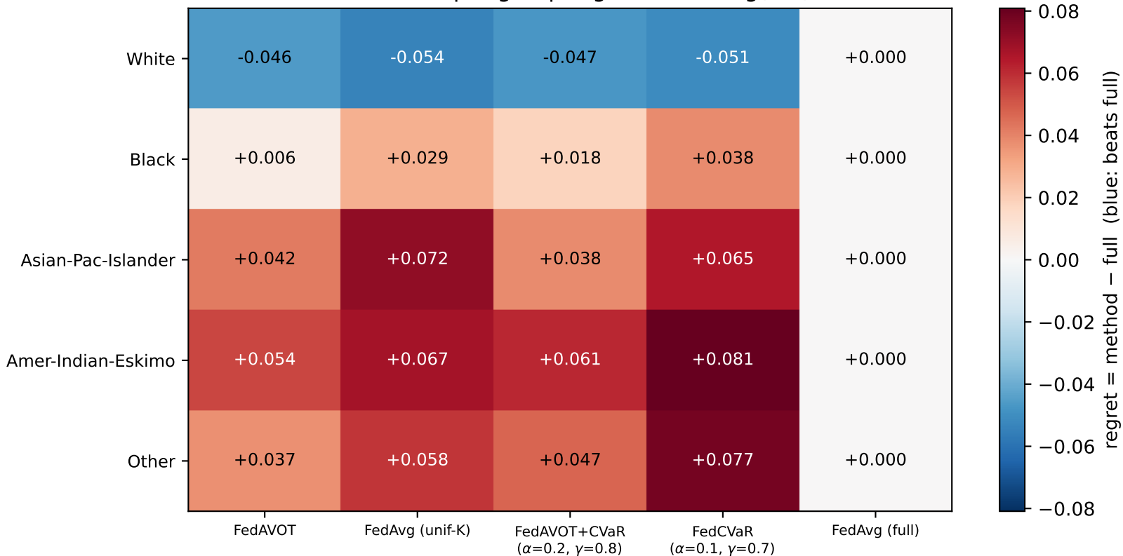
adult / infeasible — per-group regret vs FedAvg(full), tail-500
