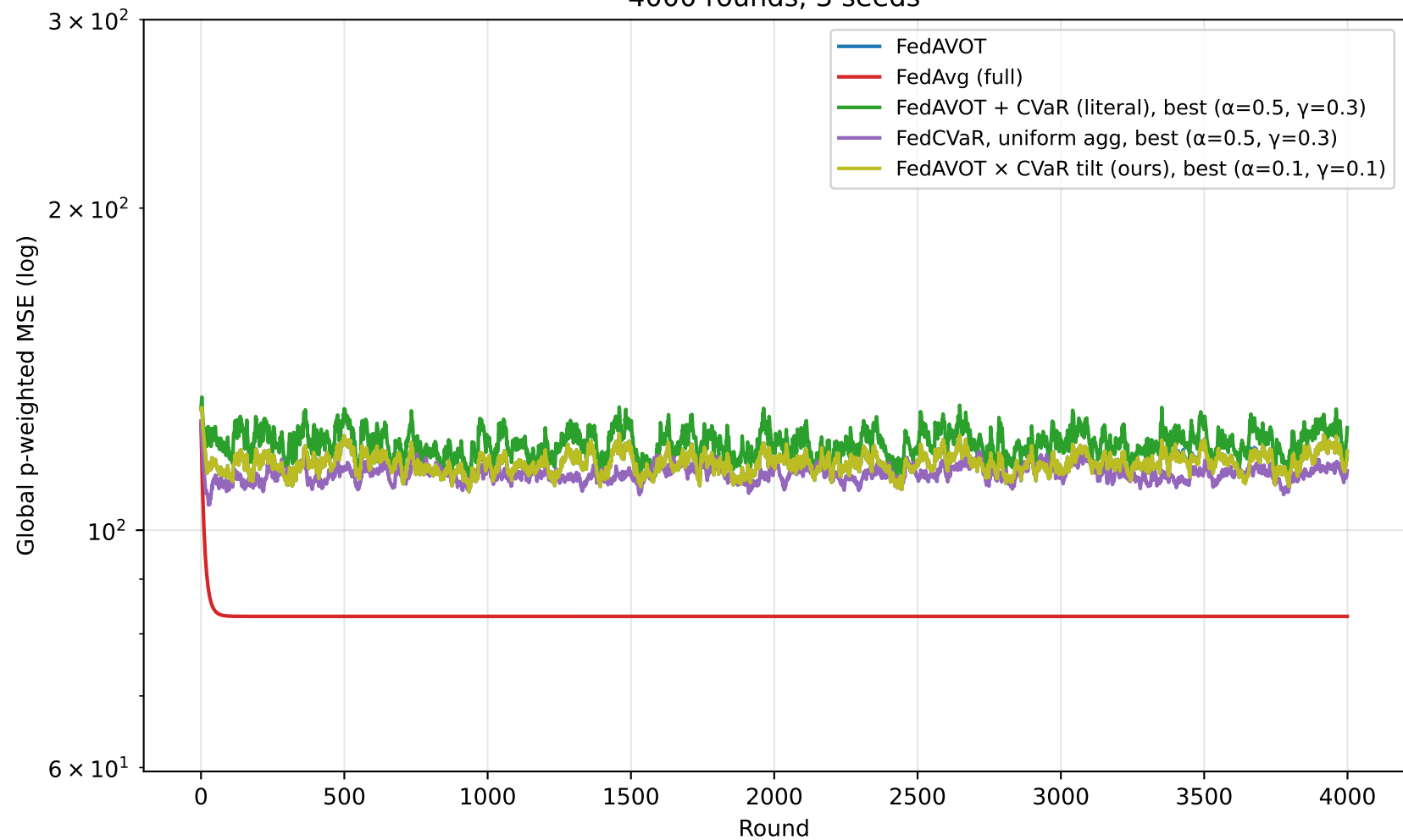
IMDb-Wiki, INFEASIBLE regime: CVaR ( \alpha, \gamma ) grid — best configs vs baselines 4000 rounds, 3 seeds
