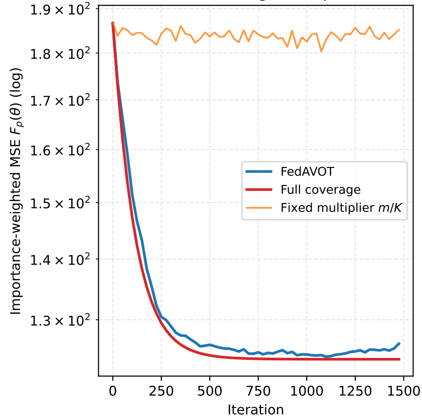
Feasible regime ( \alpha=0.5 , 14% infeasible) FedAVOT converges to optimum
