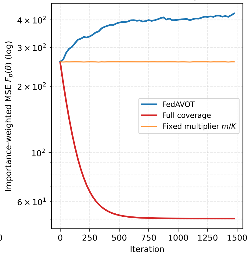
Infeasible regime ( \alpha=3.0 , 87% infeasible) FedAVOT stalls far above optimum
