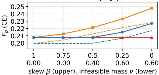
Adult, decaying \eta_t
