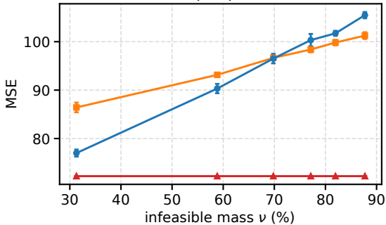
IMDb-Wiki, 20 top-importance identities
