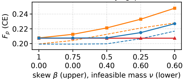
Adult, decaying \eta_t
