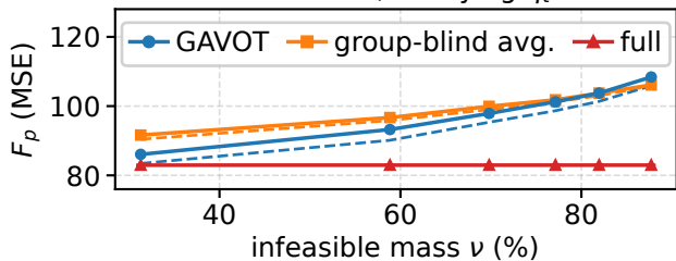
IMDb-Wiki, decaying \eta_t
