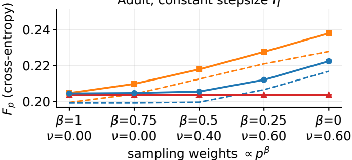
Adult, constant stepsize \eta
