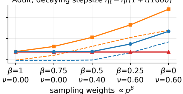
Adult, decaying stepsize \eta_t = \eta/(1 + t/1000)
