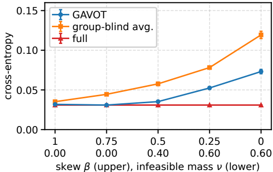
Adult, race Other
