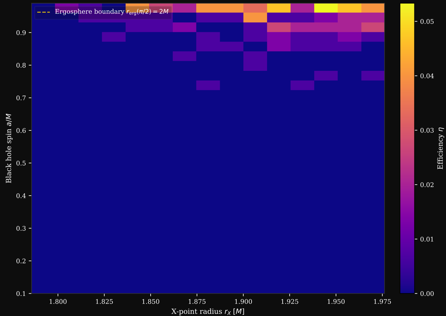
Normalized Penrose Efficiency \eta_{norm} vs Spin a/M and X-point Radius r_X
