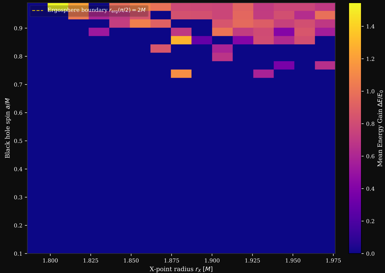
Mean Energy Gain \Delta E/E_0 vs Spin a/M and X-point Radius r_\chi
