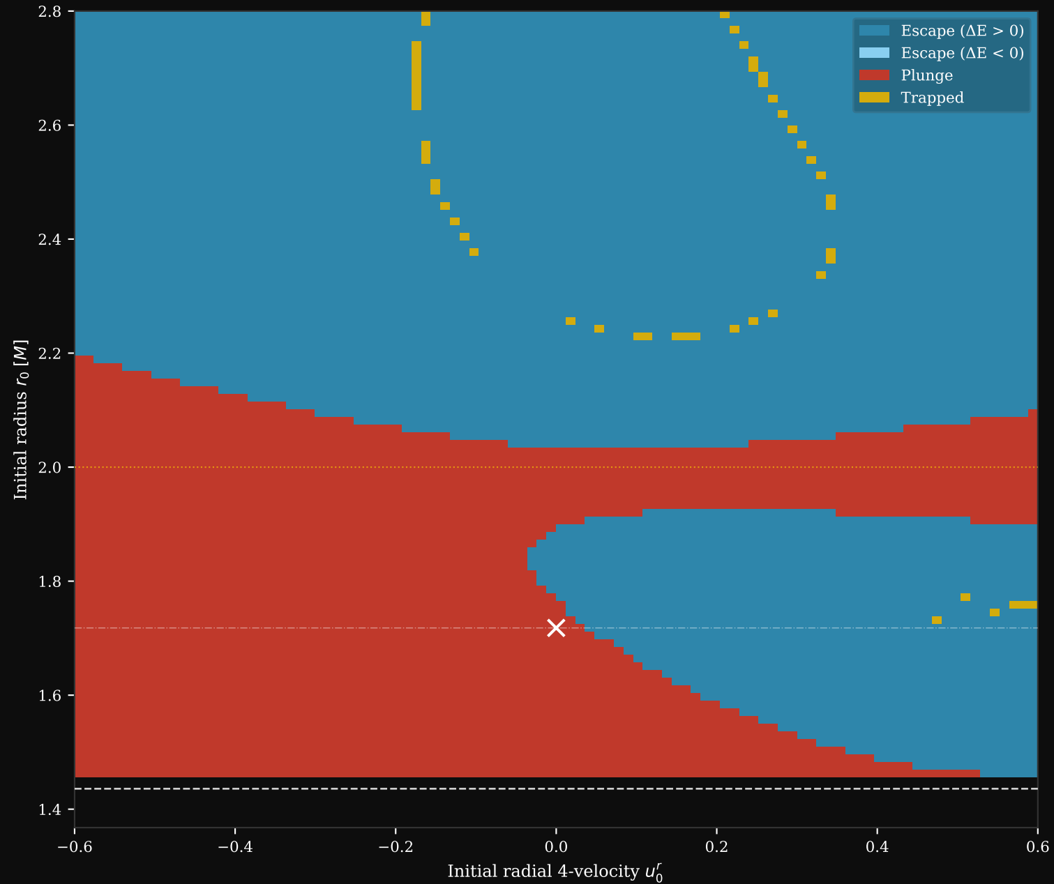
Basin of Fate ( a/M = 0.90 , B_0 = 4.0 , E_0 = 2.0 )
