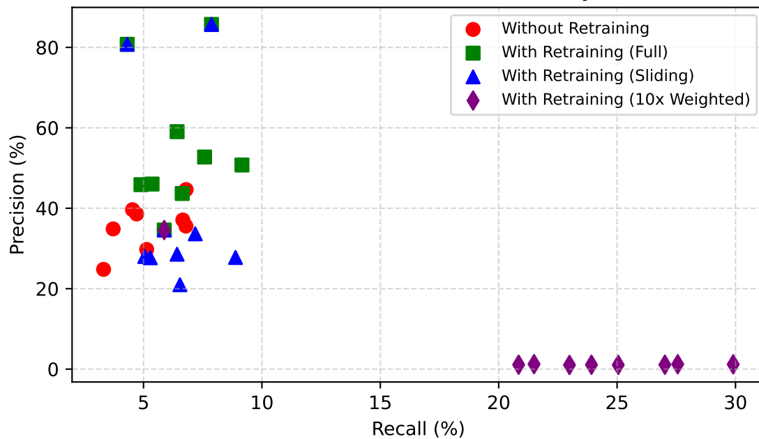
Precision vs Recall (Alert Quality)
