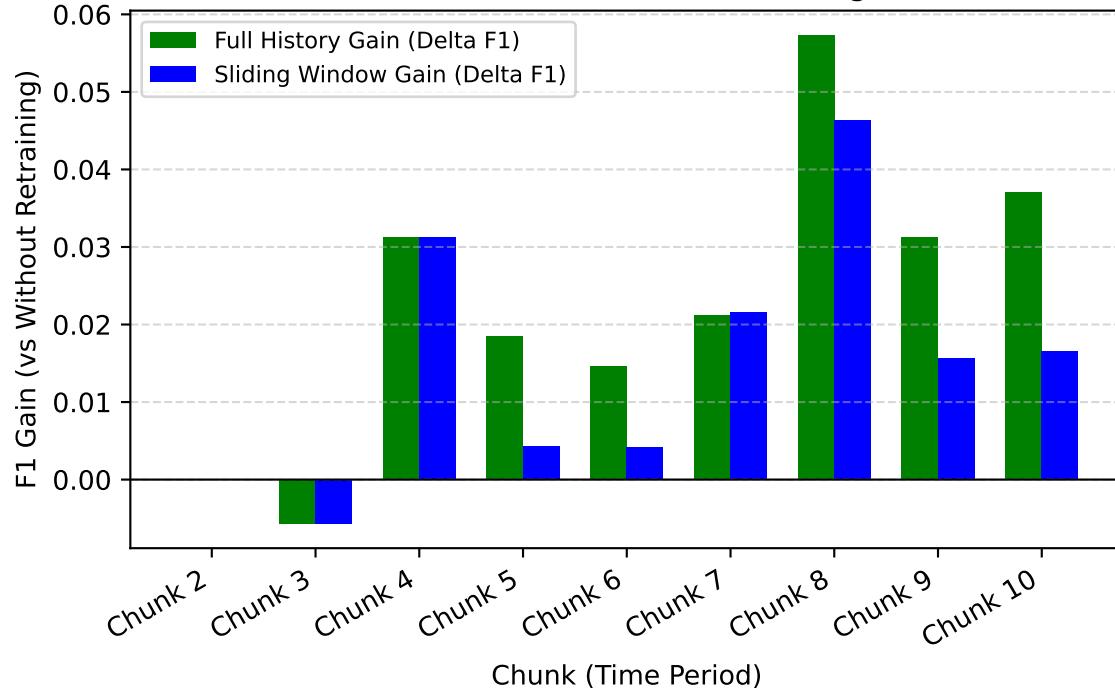
F1-Score Gain from Retraining
