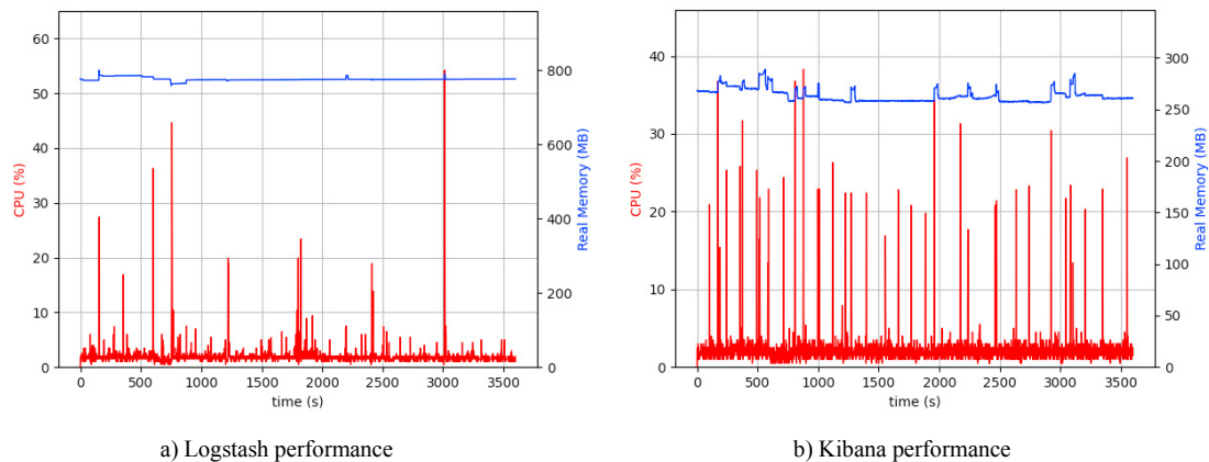
Fig 7 Logstash and Kibana performance.
