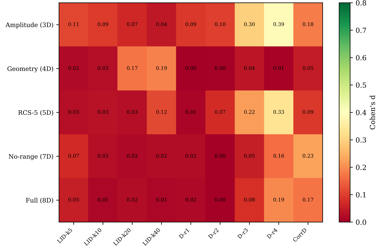
(a) Cargo-Tanker Cohen's d per subspace \times feature (green = high separation; red line = 0.56 ceiling)
