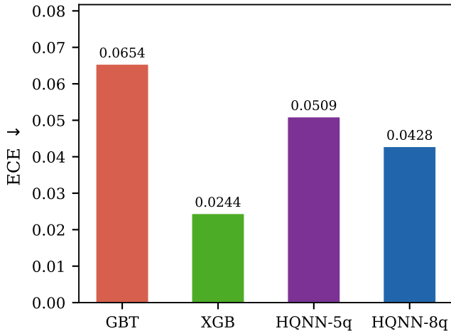
(b) Expected Calibration Error
