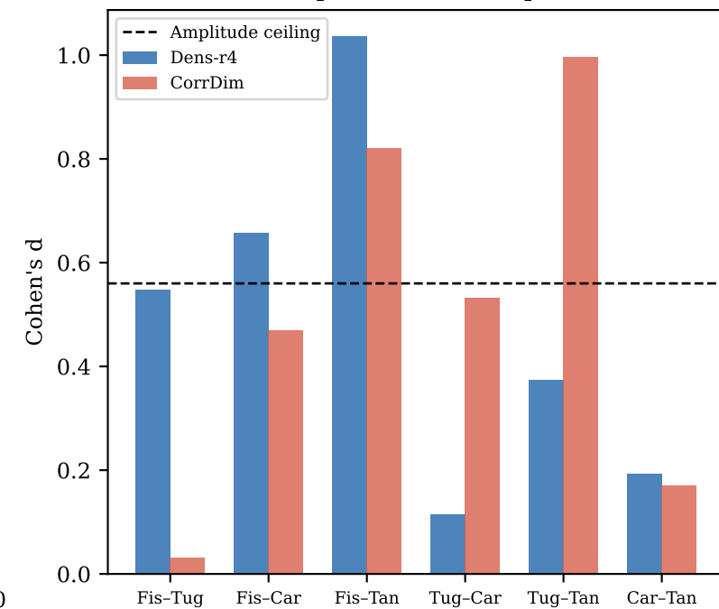
(c) Top-2 features all pairs
