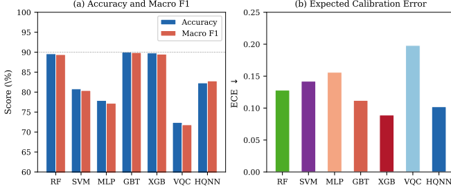
Fig. 1: Full model comparison across classical and quantum architectures. (a) Accuracy and Macro F1; GBT and RF lead on raw accuracy. (b) Expected Calibration Error (ECE): XGB and HQNN show superior probability calibration despite lower accuracy than GBT.
