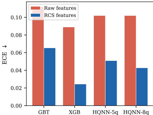
(a) ECE: raw vs RCS features
