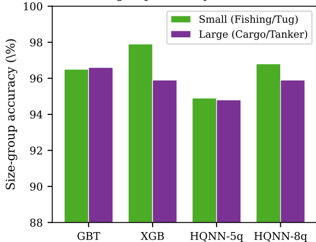
(b) Size-group accuracy (RCS features)
