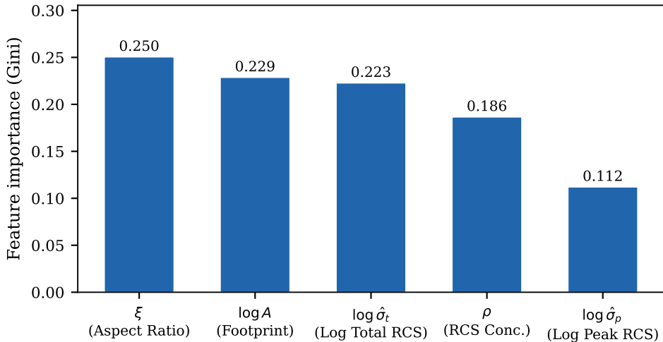
GBT feature importance — RCS feature set
