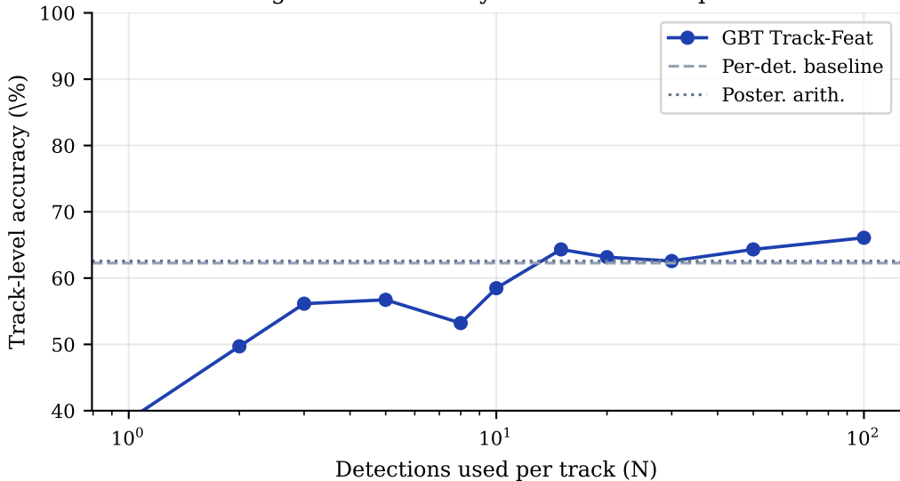
Learning Curve: Accuracy vs N Detections per Track
