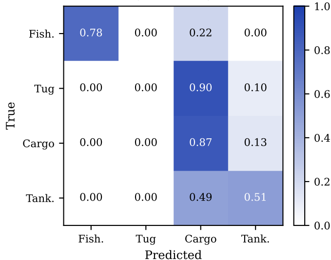
GBT Track-Feat (acc=0.702)
