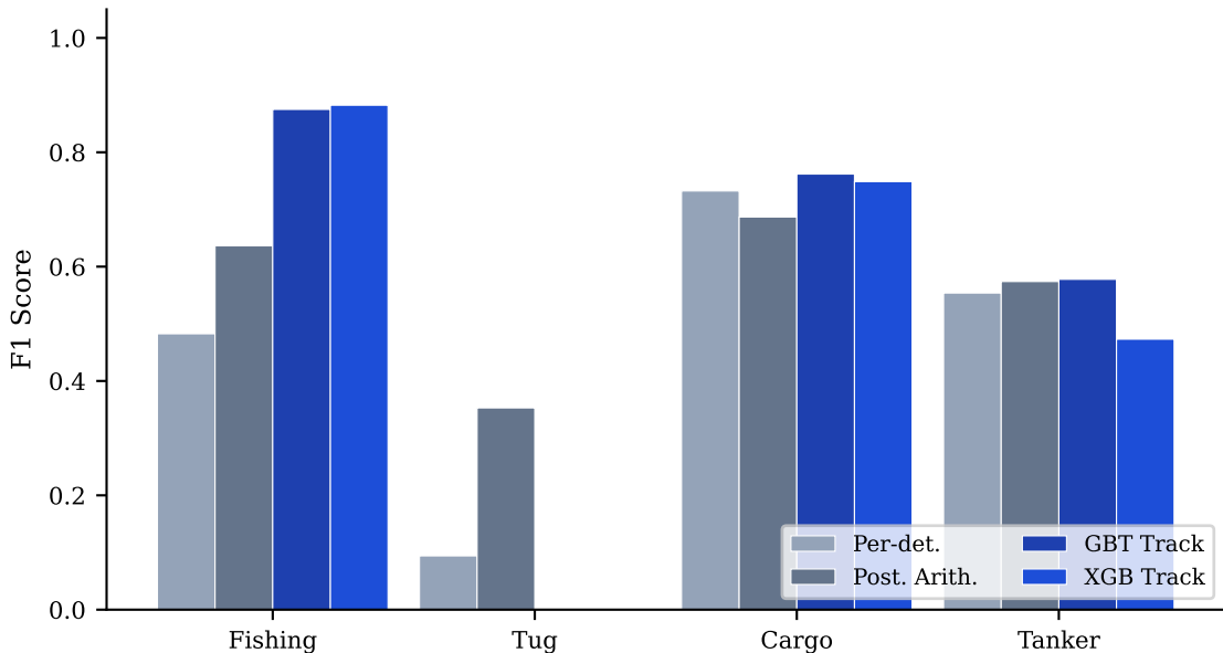
Per-Class F1: Detection-Level vs Track-Level Feature Engineering
