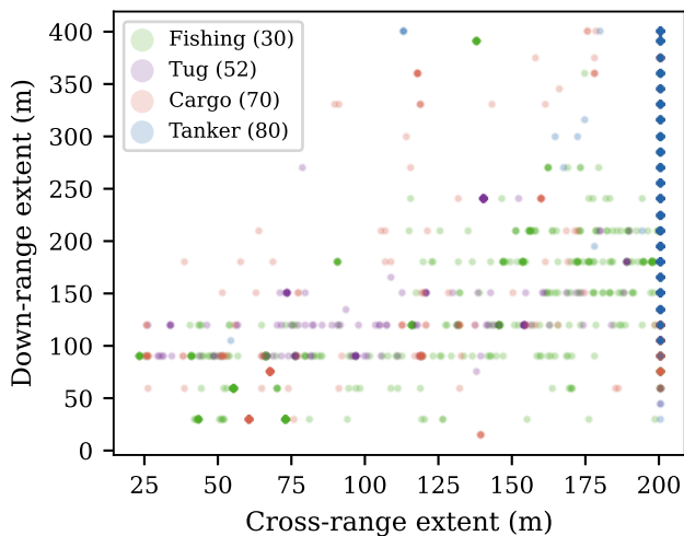
(b) Radar footprint by vessel type
