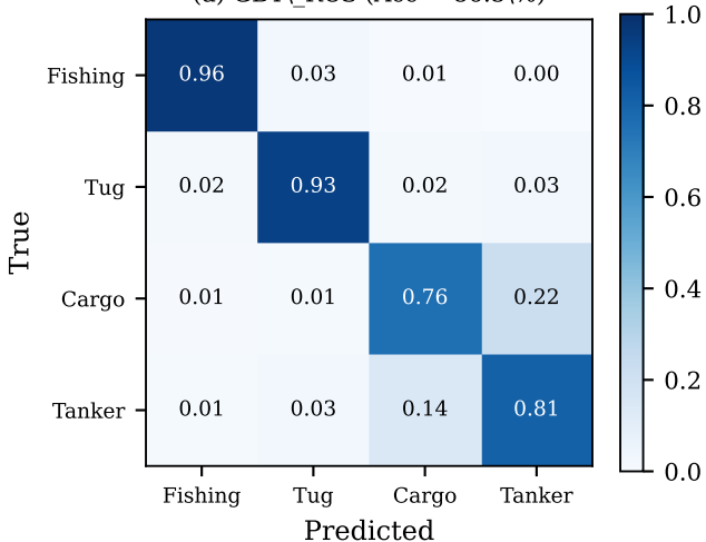
(a) GBT\RCS (Acc = 86.5\%)
