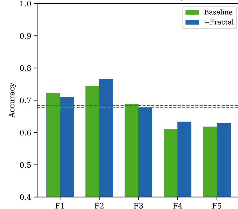
(c) Per-fold accuracy
