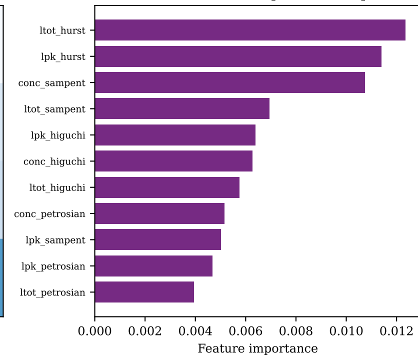
(f) Fractal feature importance (top 11)
