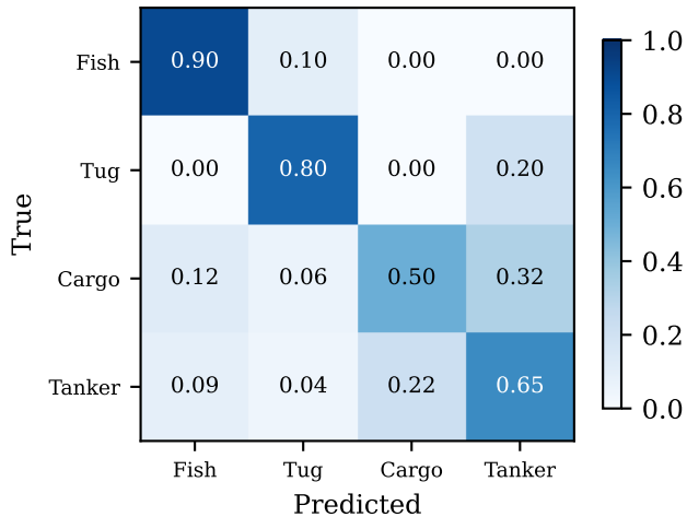
(b) BiLSTM-v2 confusion (per-track)
