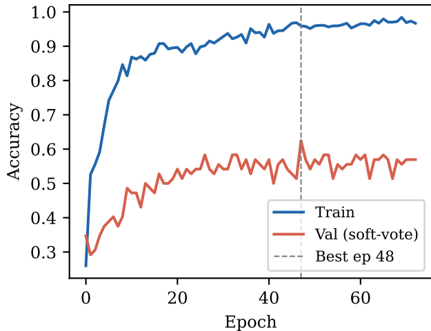
(a) BiLSTM-v2 learning curves
