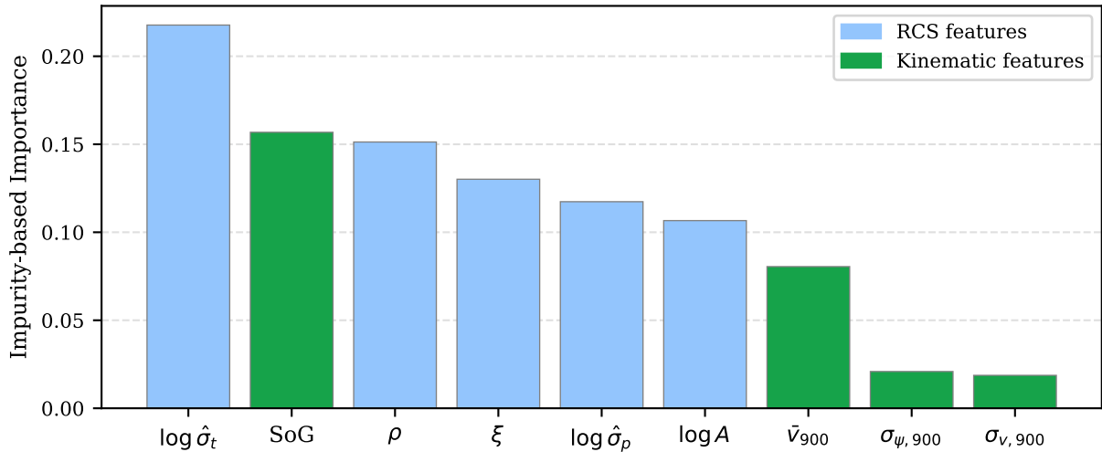
Figure 4: GBT Feature Importance — Kinematic+RCS (9 features)
