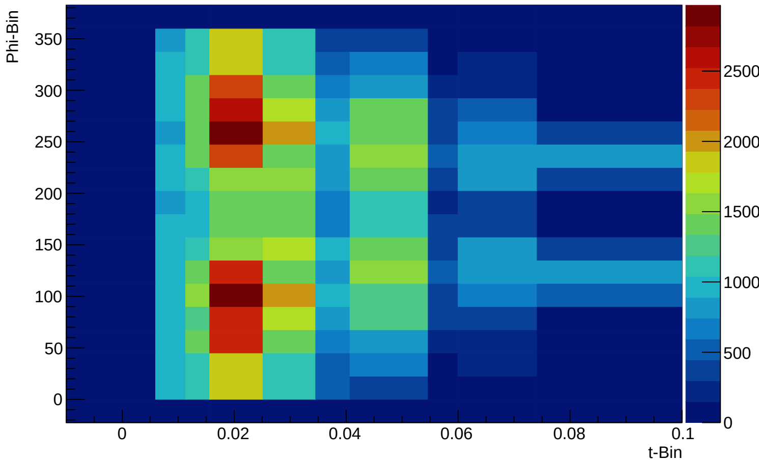
Total Yield for High epsilon
