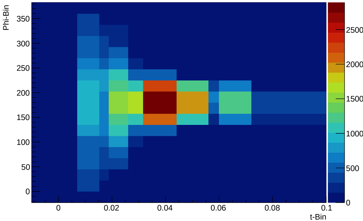
Total Yield for low epsilon
