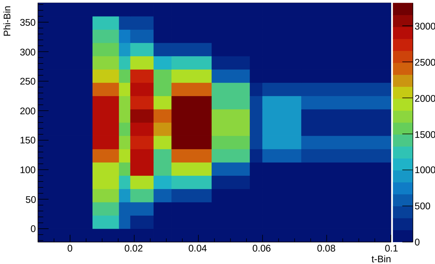
Total Yield for mid epsilon
