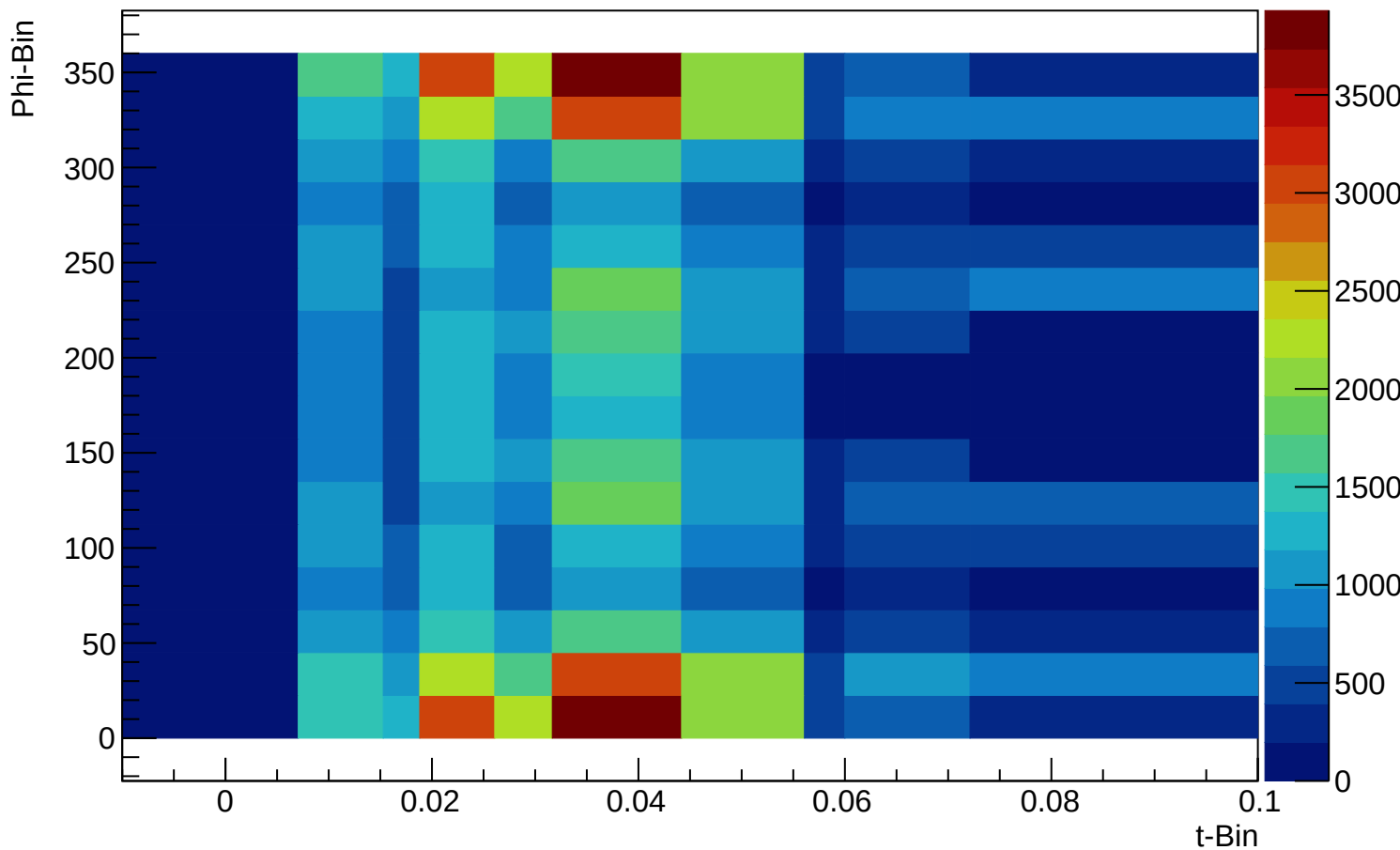
Total Yield for High epsilon
