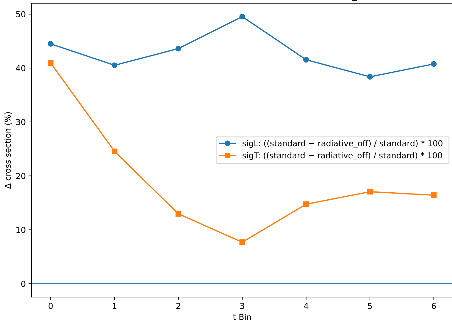
Radiative Correction Effect (Standard – Radiative_off)
