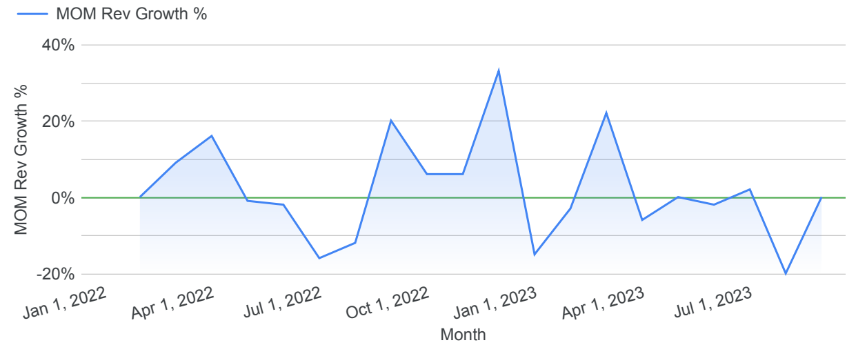
MOM Rev Growth % by Month
