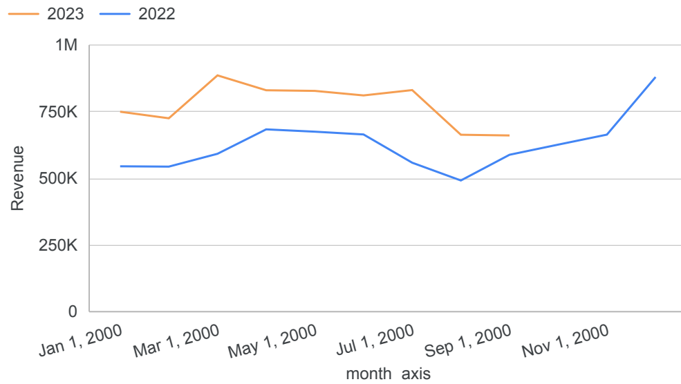
Monthly Revenue — Year-over-Year Comparison
