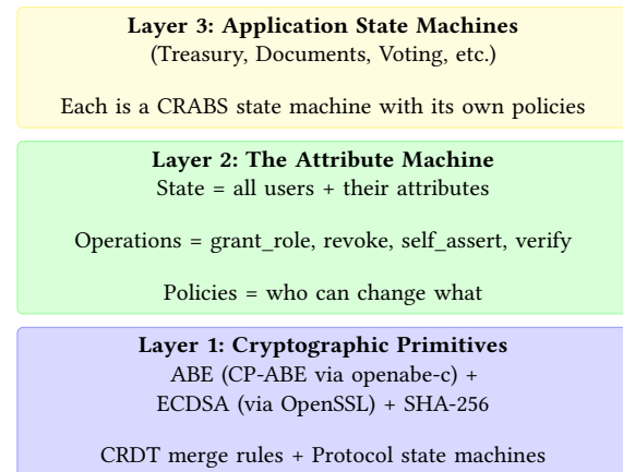
Figure 1: The three-layer CRABS architecture. The Attribute Machine is the foundation; application machines reference its state for authorization decisions.
