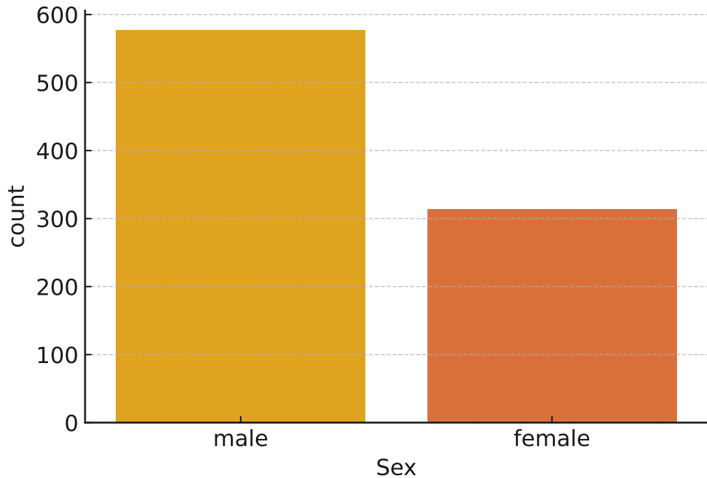
Gender Count
