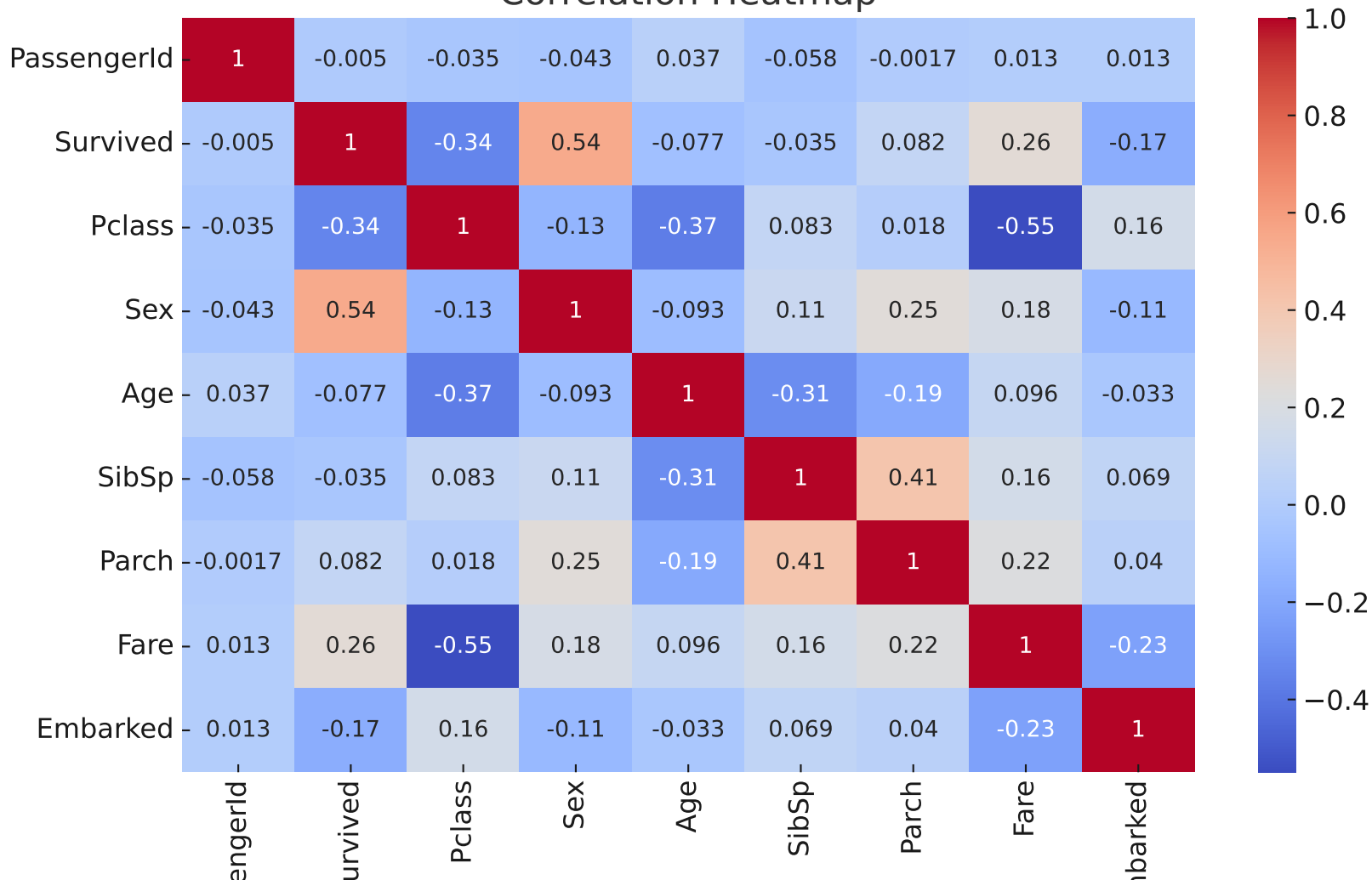
Correlation Heatmap
