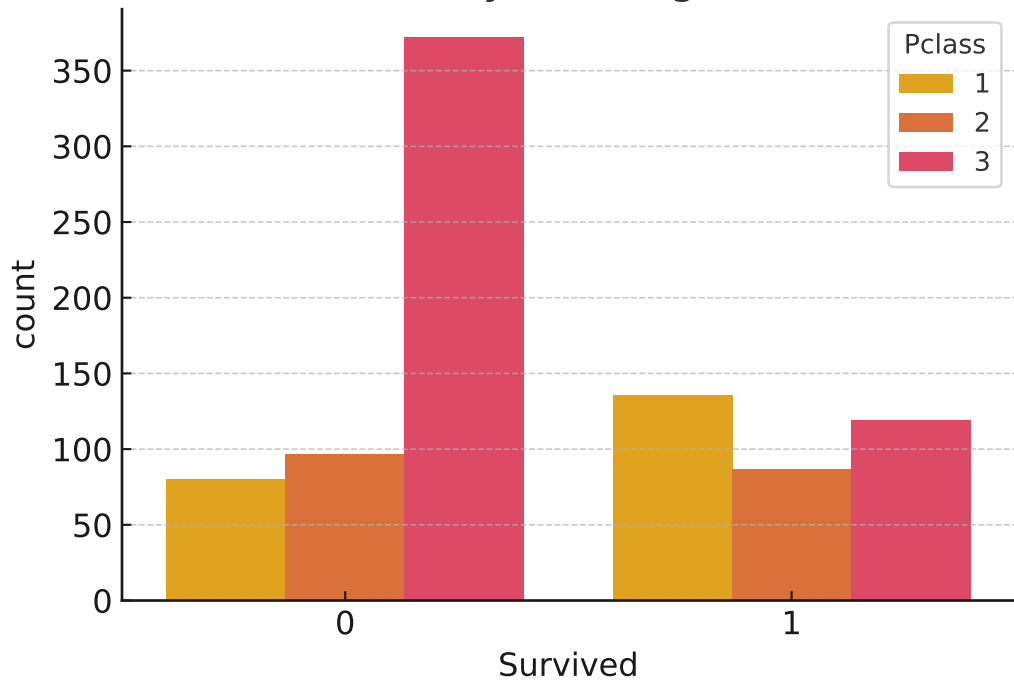
Survival by Passenger Class
