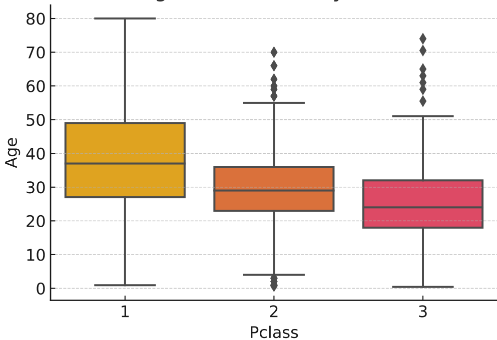
Age Distribution by Class
