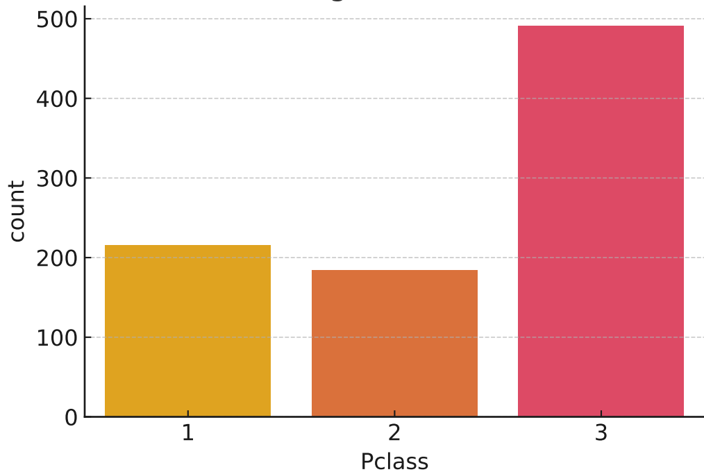
Passenger Class Count
