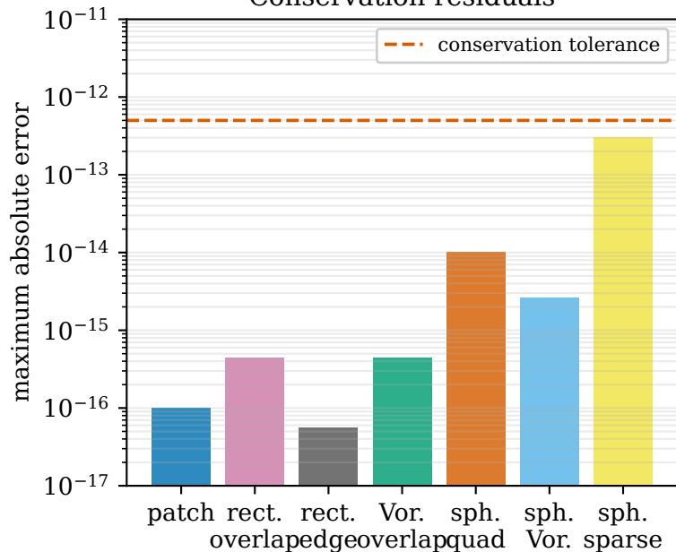
Conservation residuals
