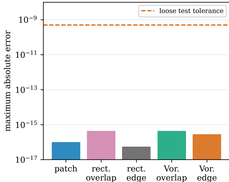
Conservation residuals
