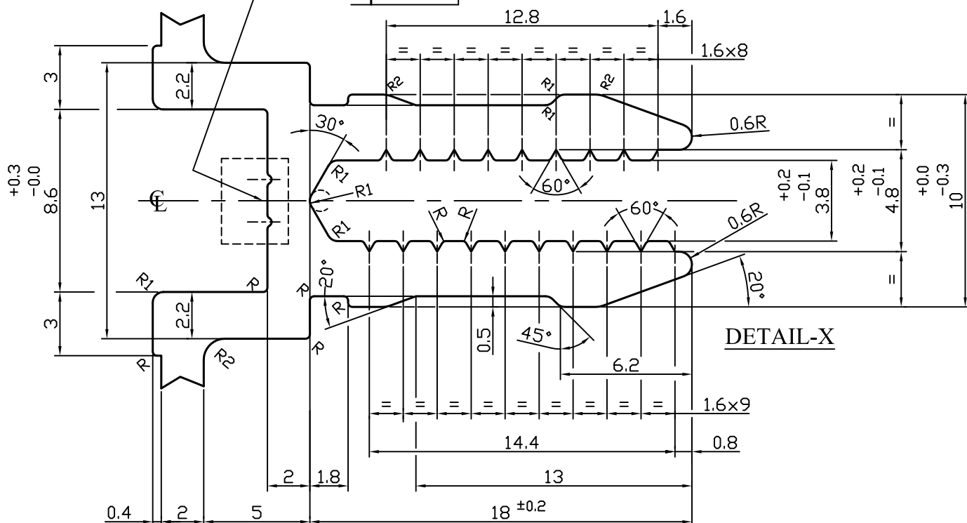
DETAILS OF SECTION 14716
