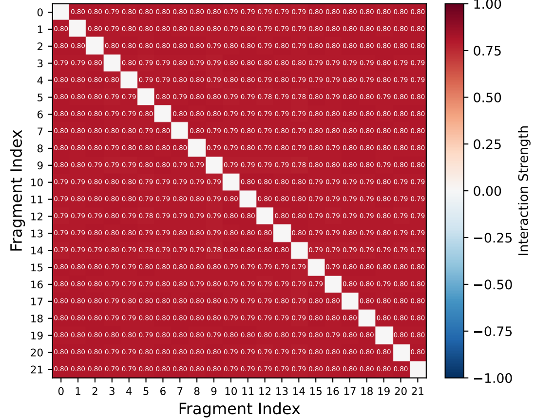
(c) Association Matrix \theta
