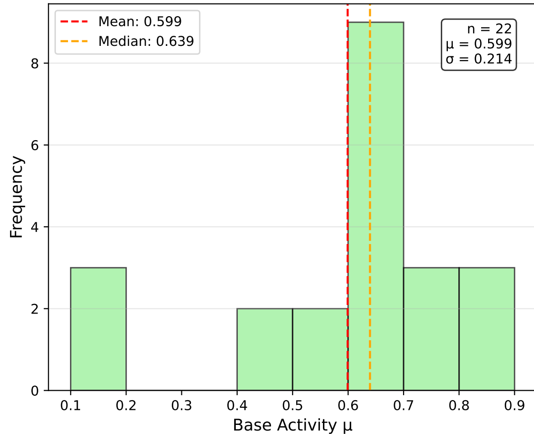
(b) Base Activities \mu Distribution
