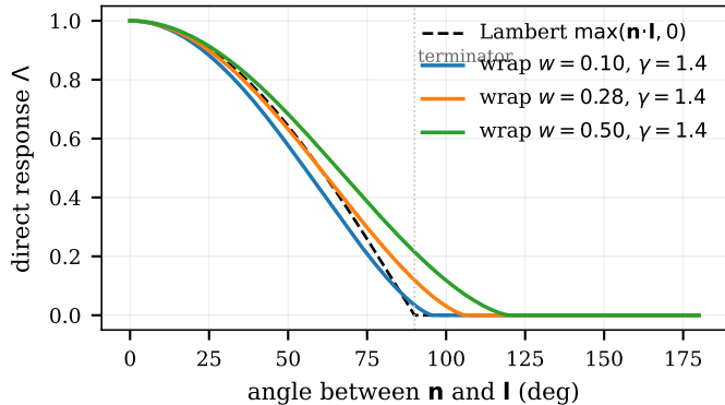
wrapped Lambert falloff
