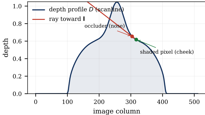
screen-space cast shadow test
