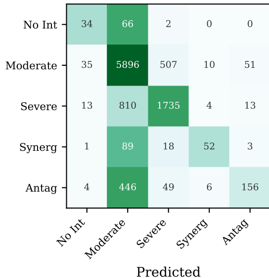
Argmax Severe recall = 0.674
