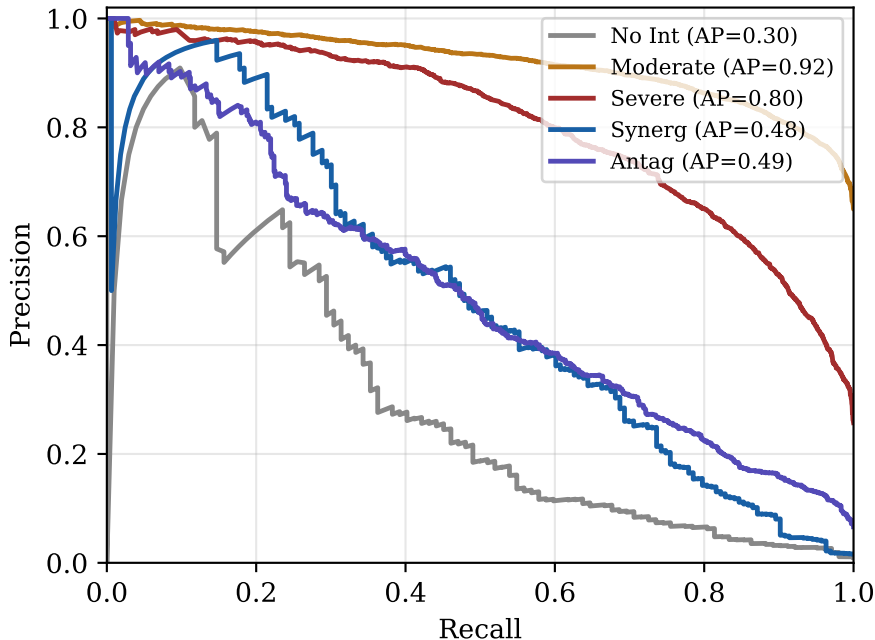
Per-class precision-recall curves
