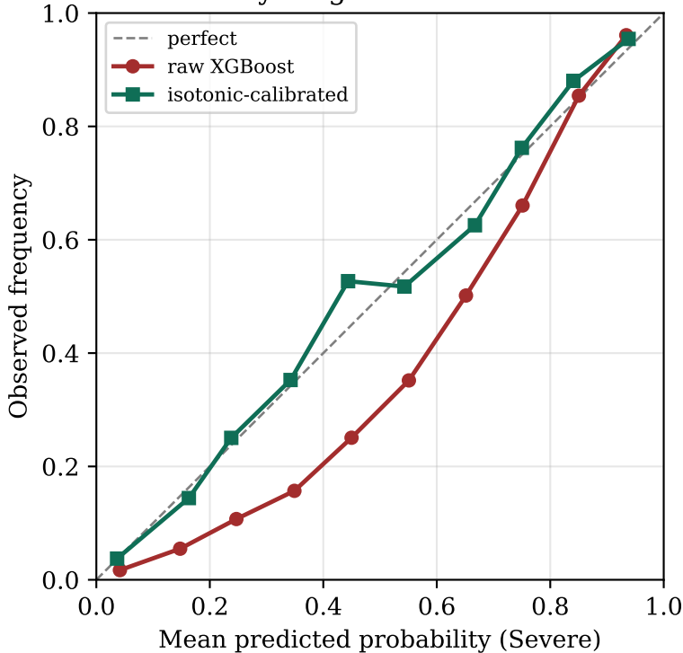
Reliability diagram — Severe class
