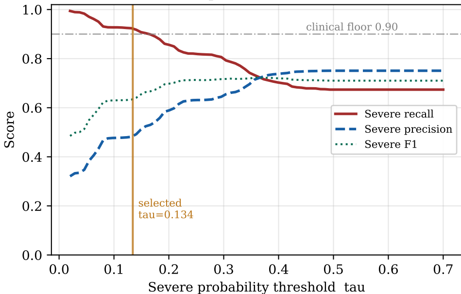
Severe-class recall/precision vs. decision threshold
