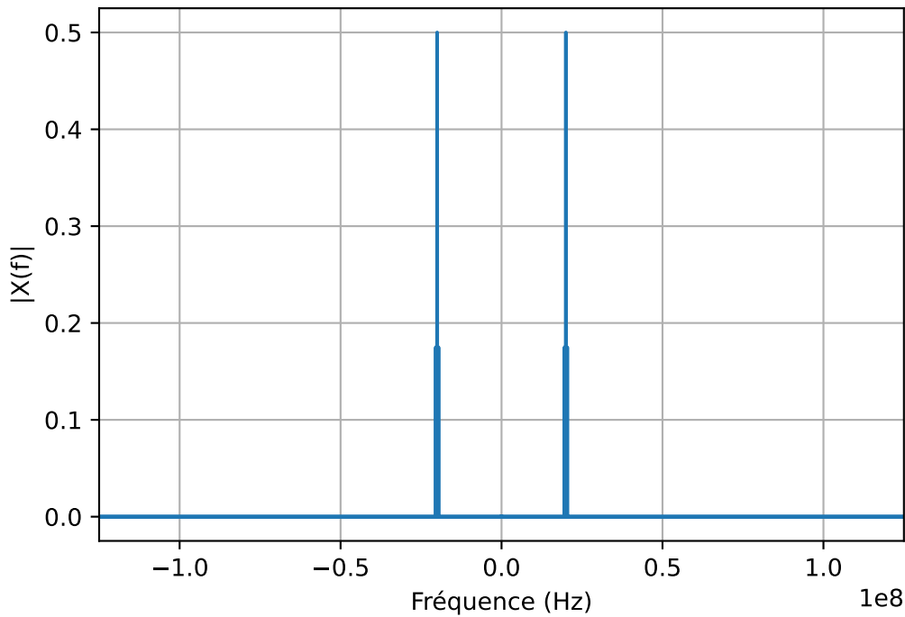
Spectre du signal A3
