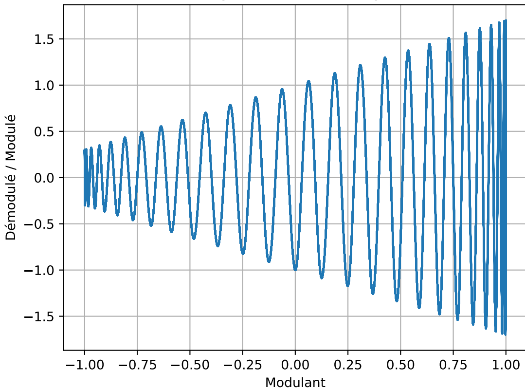
A3 — X-Y : signal modulant vs signal modulé
